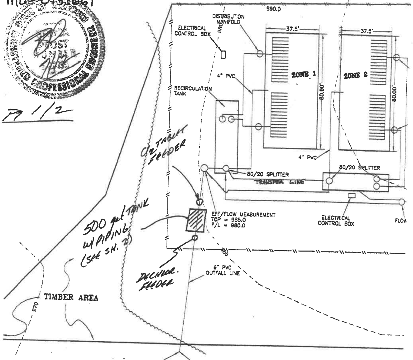
SITE PLAN
