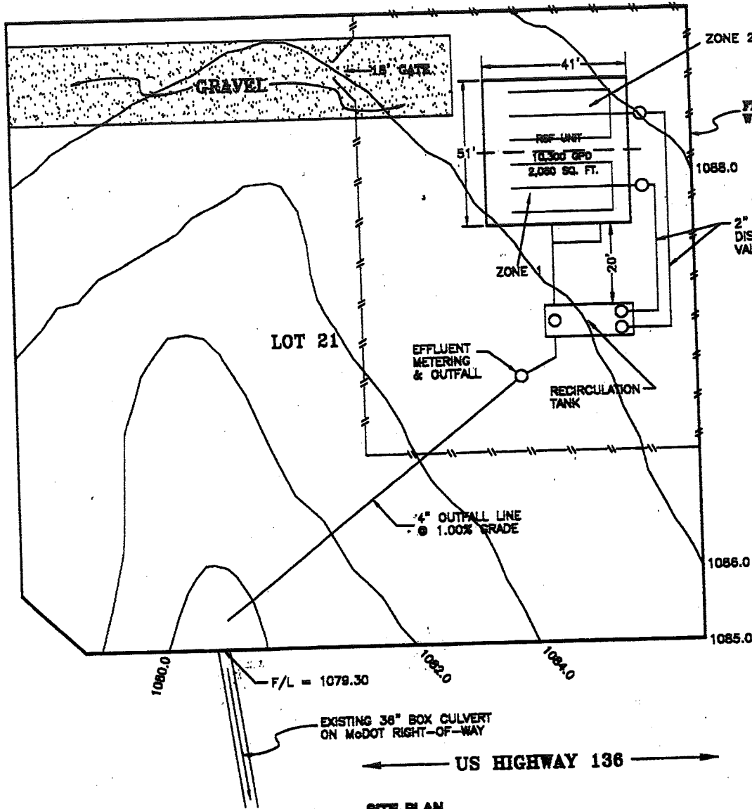
SITE PLAN NO SCALE
