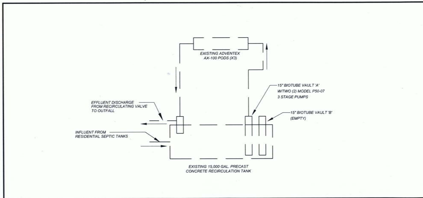
PROCESS FLOW DIAGRAM NOT TO SCALE
