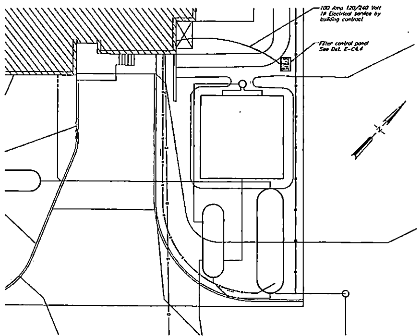
D SITE ELECTRICAL Scale: 1" = 10'
