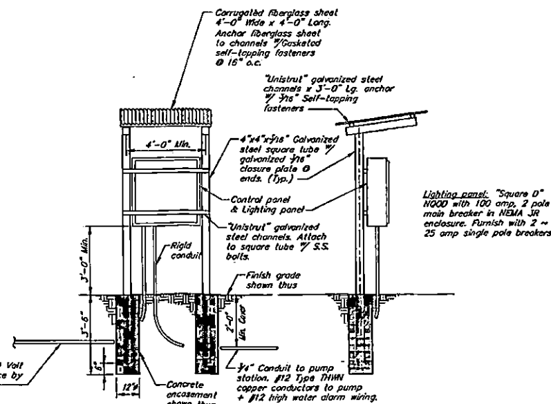
E ELECTRICAL/CONTROL PANEL DETAIL
