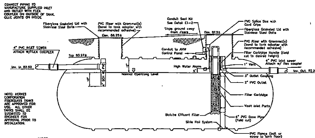
B 10,000 GAL. PRIMARY TANK (8'0" x 31.5' Long)
