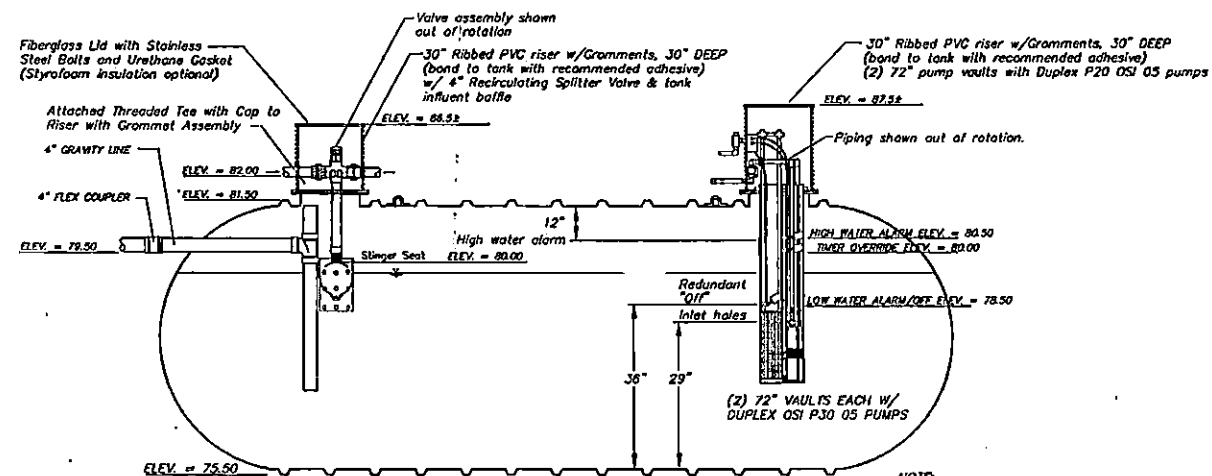
C 4,000 GAL. RECIRCULATION TANK (6'0" x 22' Long)
