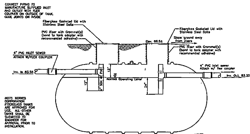
A 2000 GAL. KITCHEN HOLDING TANK (8'0" x 13.5' Long)
