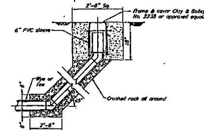
G STANDARD CLEANOUT DETAIL n.l.s.
