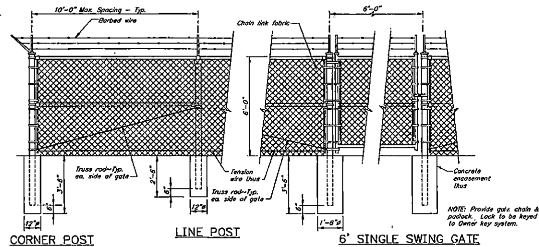
F FENCE AND GATE DETAIL Scale: 1/2" = 1'-0"
