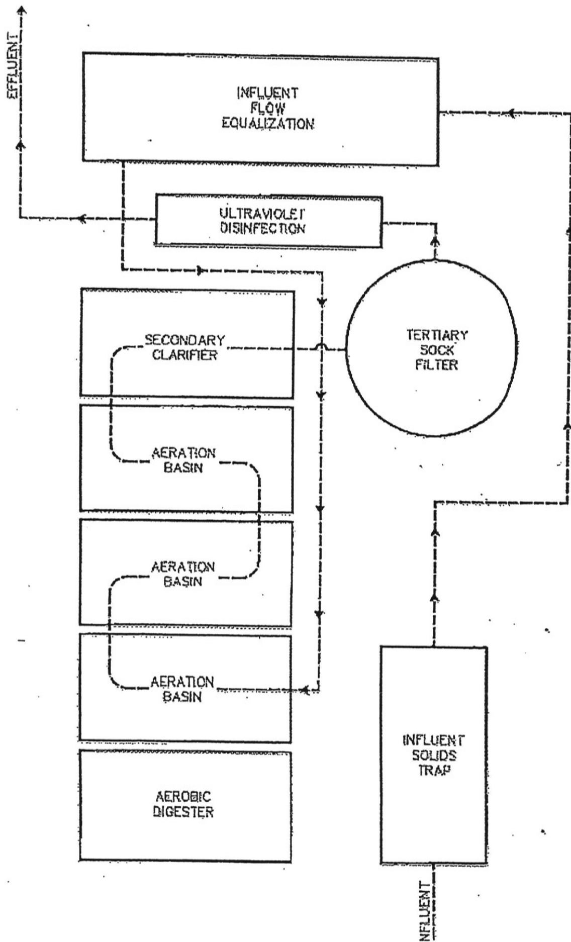
APPENDIX – ALTERNATIVE: PROCESS FLOW DIAGRAM FOR RSD, ROCKWOOD VALLEY MIDDLE SCHOOL WWTF
