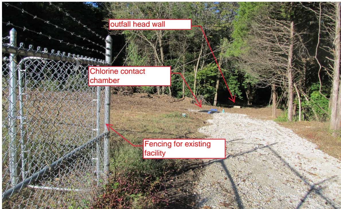
New access to facility and chlorine contact chamber.
