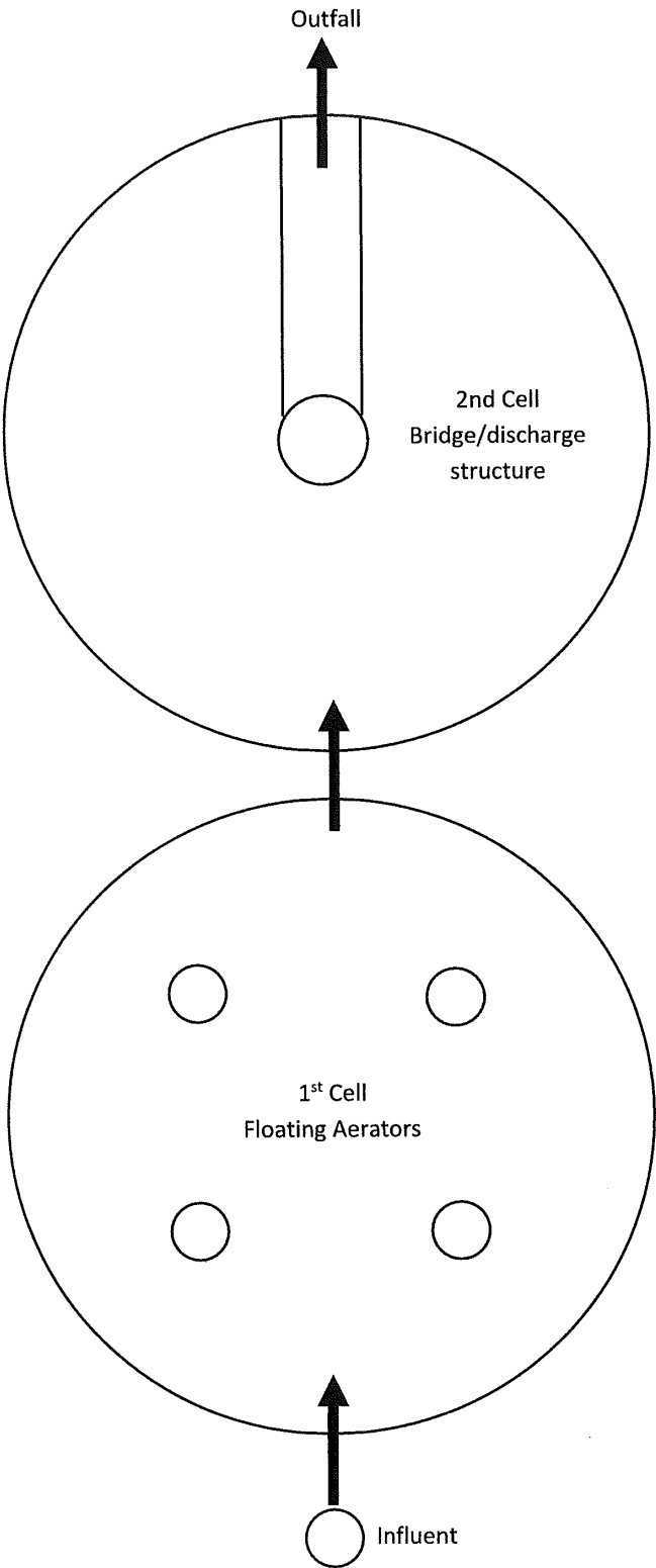
City of High Hill WWTF – Flow Diagram
