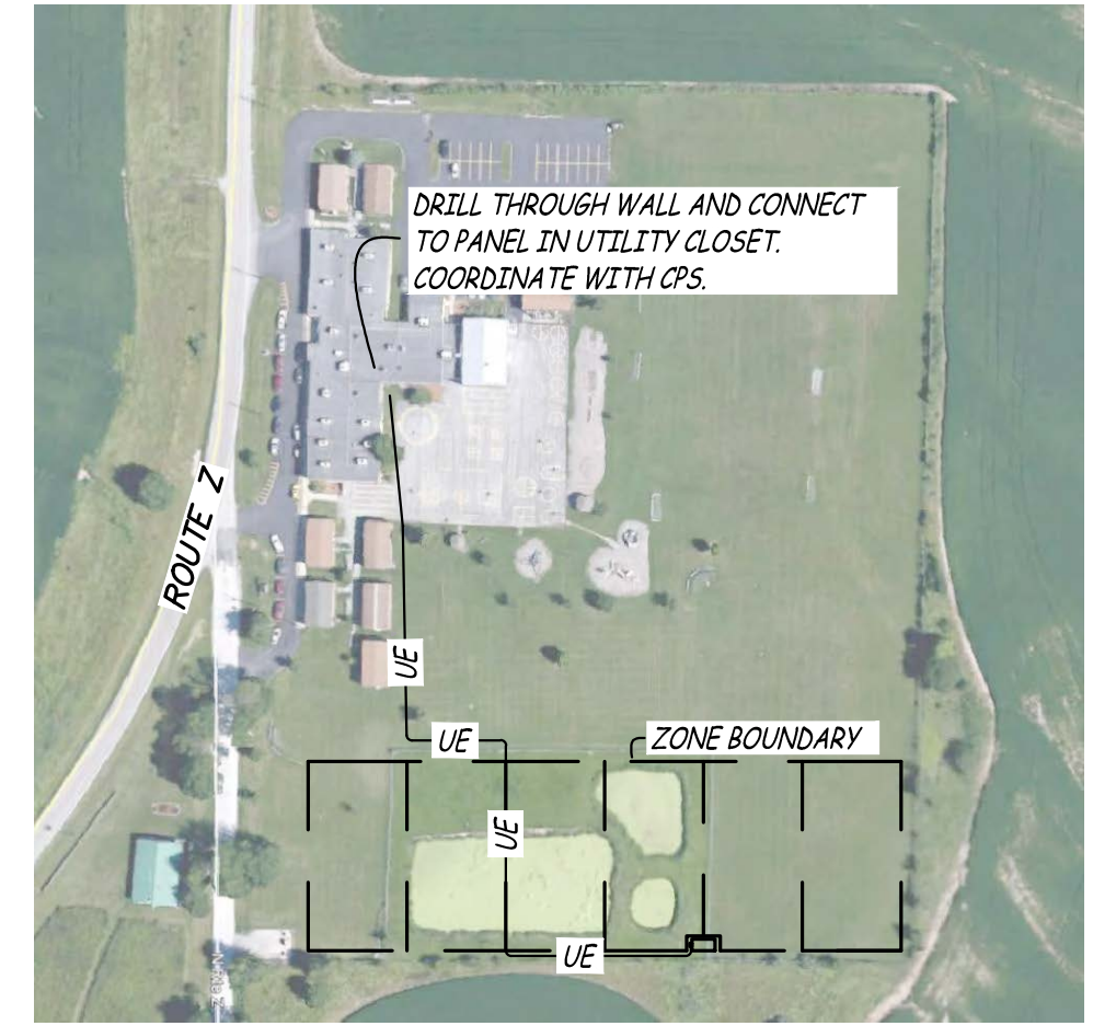
ELECTRICAL ROUTE SCALE: 1"=200'
