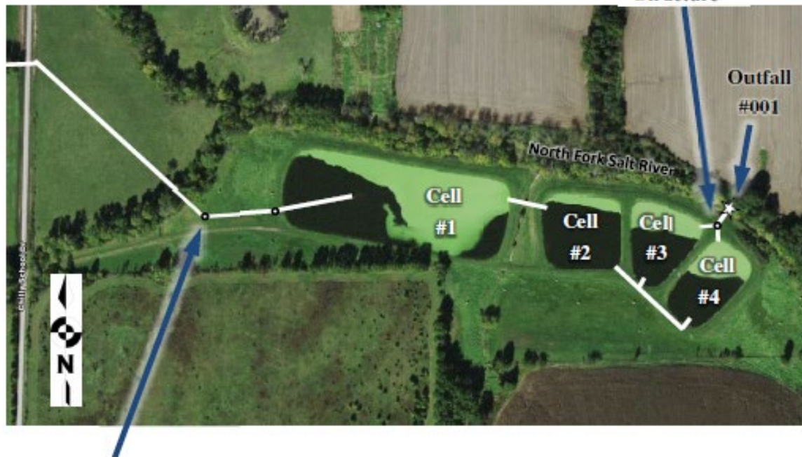
Influent Flow Meter Structure
