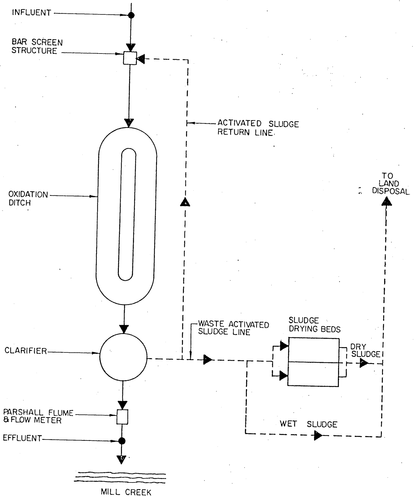
Figure No. 1 Basic Flow Diagram
