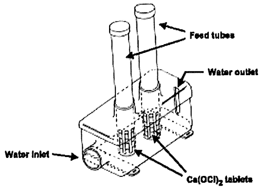
Schematic of Typical Tablet Style Chlorinator and Dechlorinator
