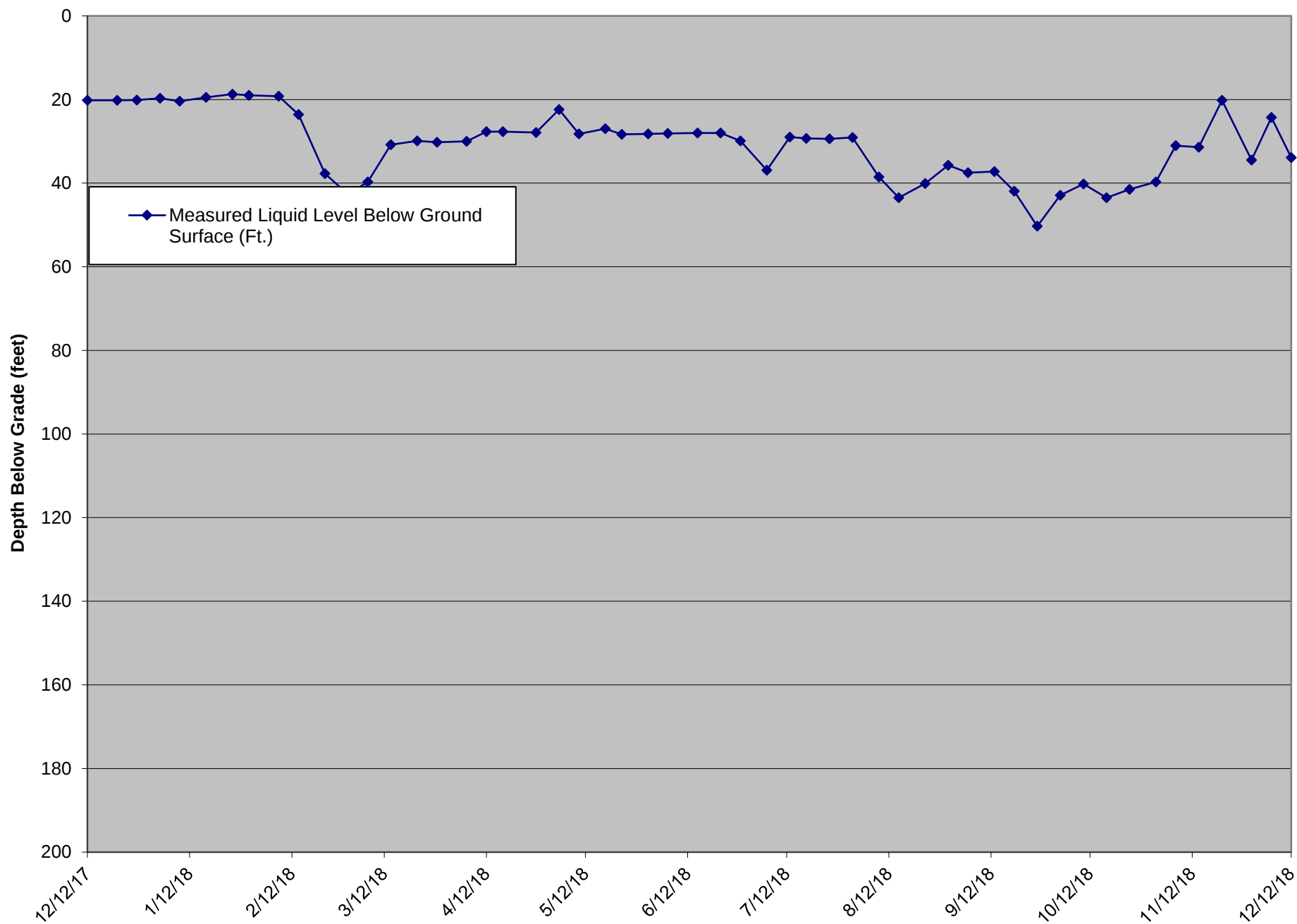
LCS-3D Liquid Level Below Ground Surface
