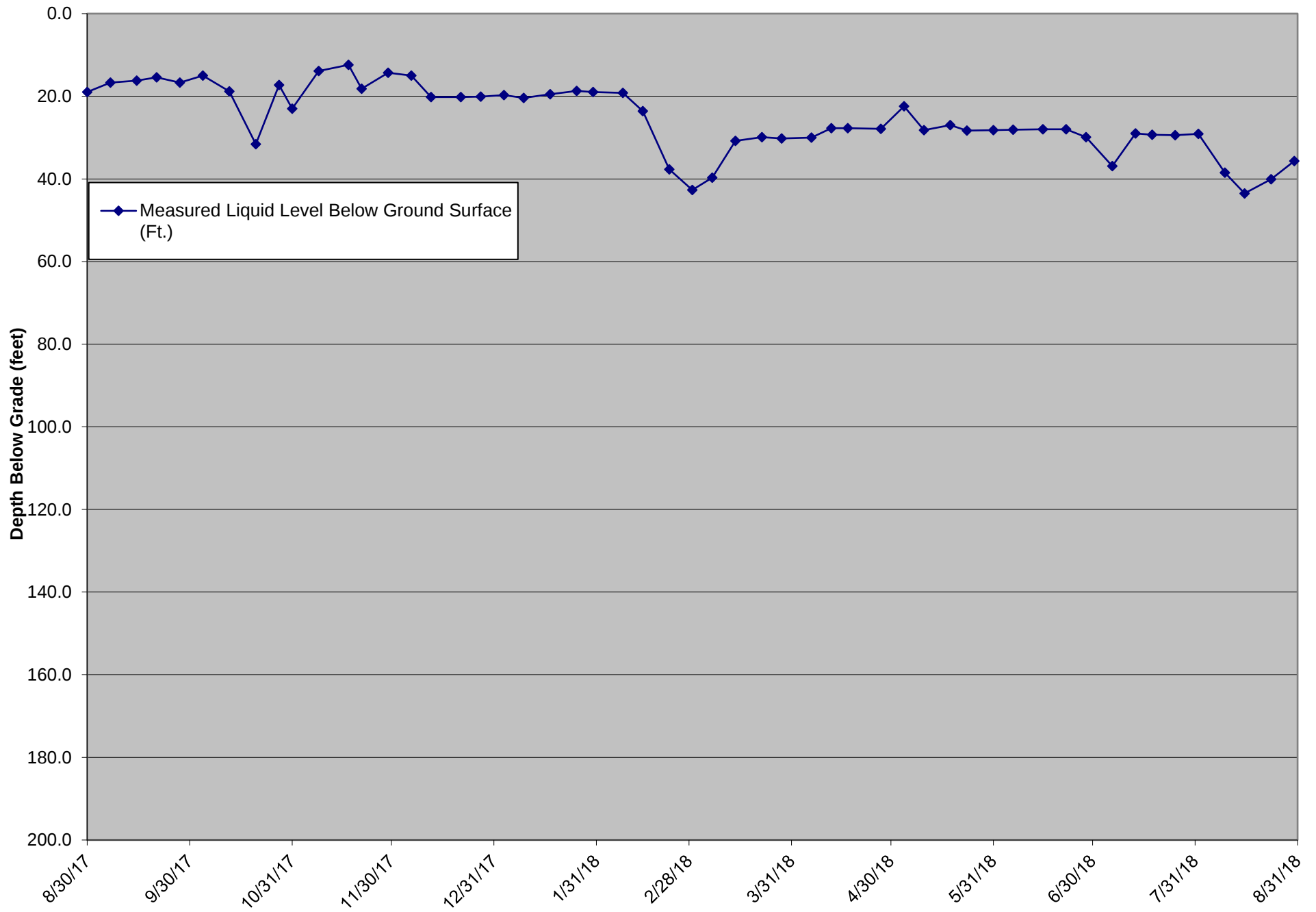
LCS-3D Liquid Level Below Ground Surface
