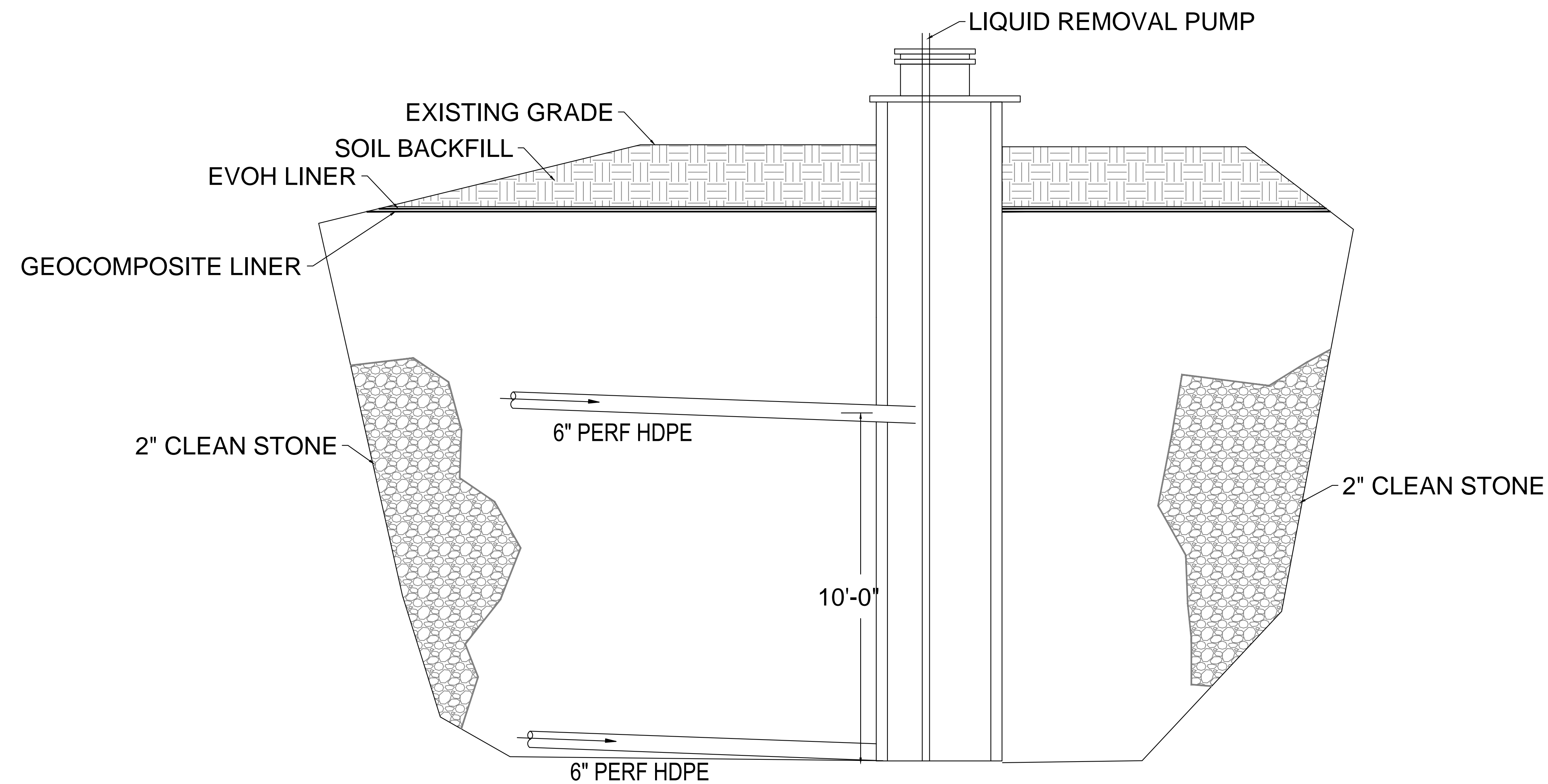
SECTION A-A NTS
