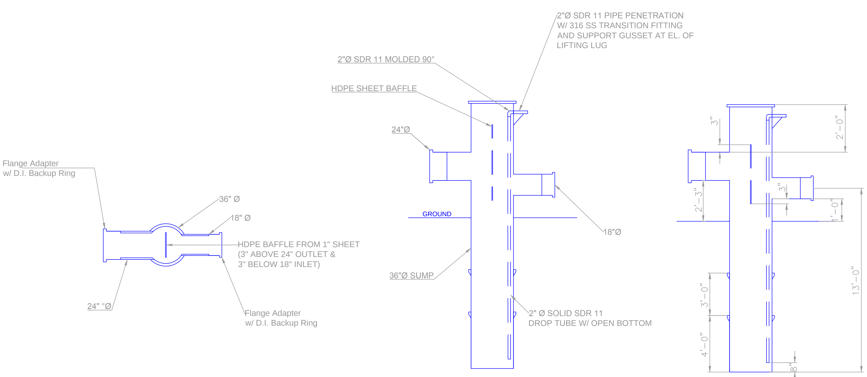
CONDENSATE SUMP 31 NOT TO SCALE
