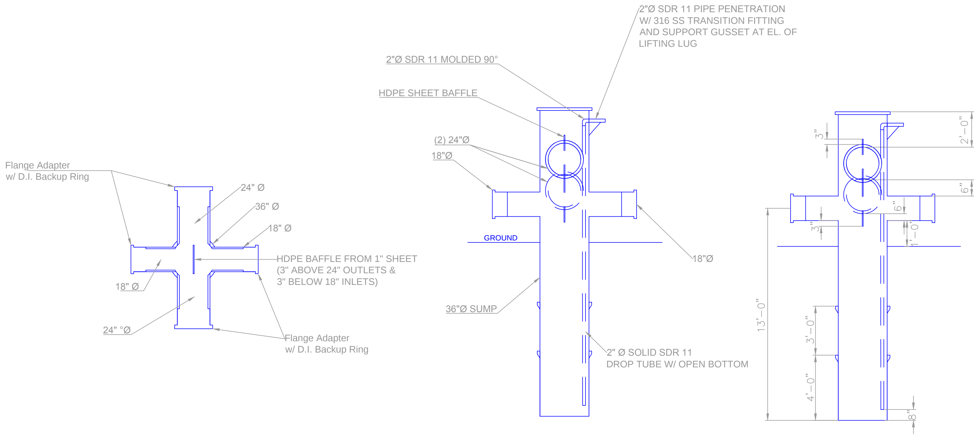
CONDENSATE SUMP 81 NOT TO SCALE
