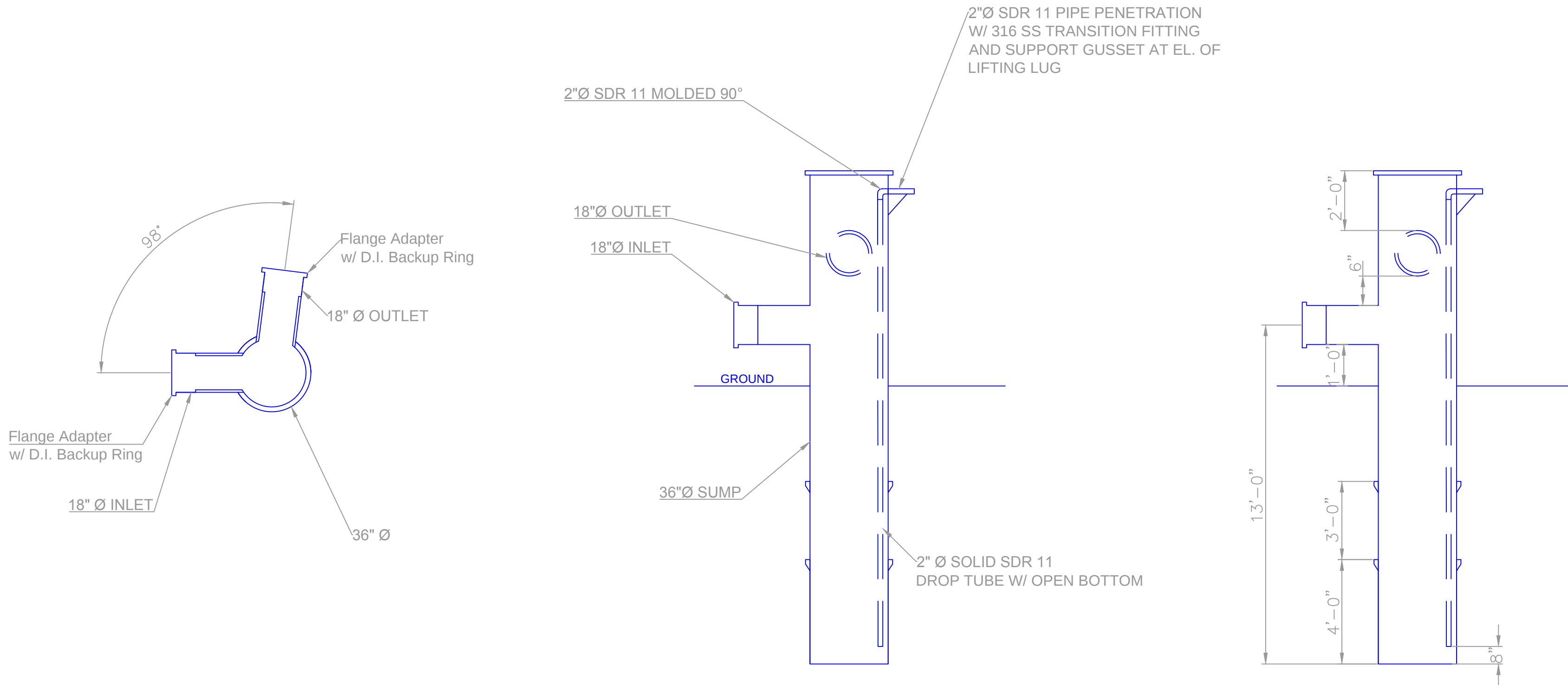
CONDENSATE SUMP 33 NOT TO SCALE
