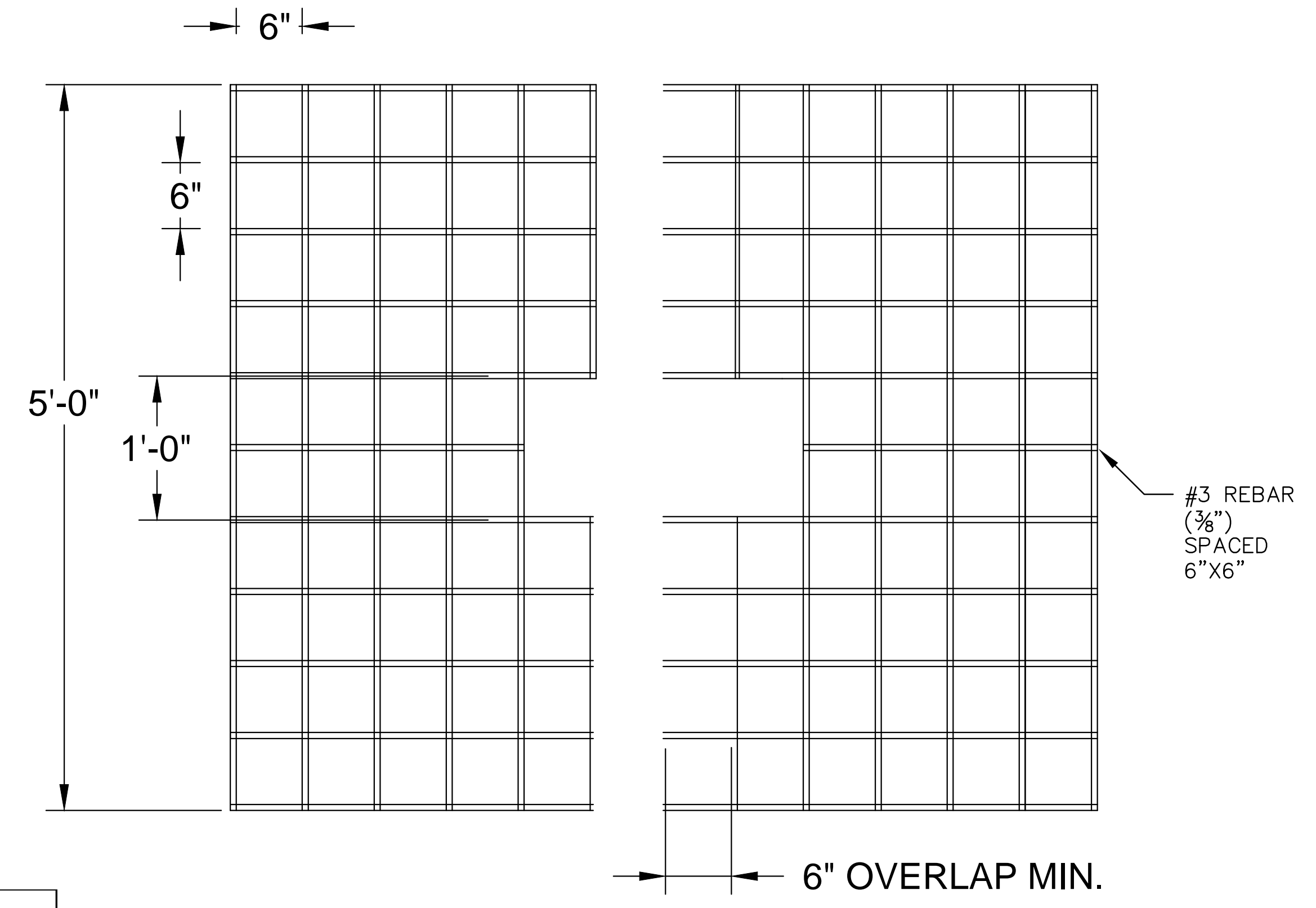
4 WELL BORE REINFORCEMENT GRATE NOT TO SCALE
