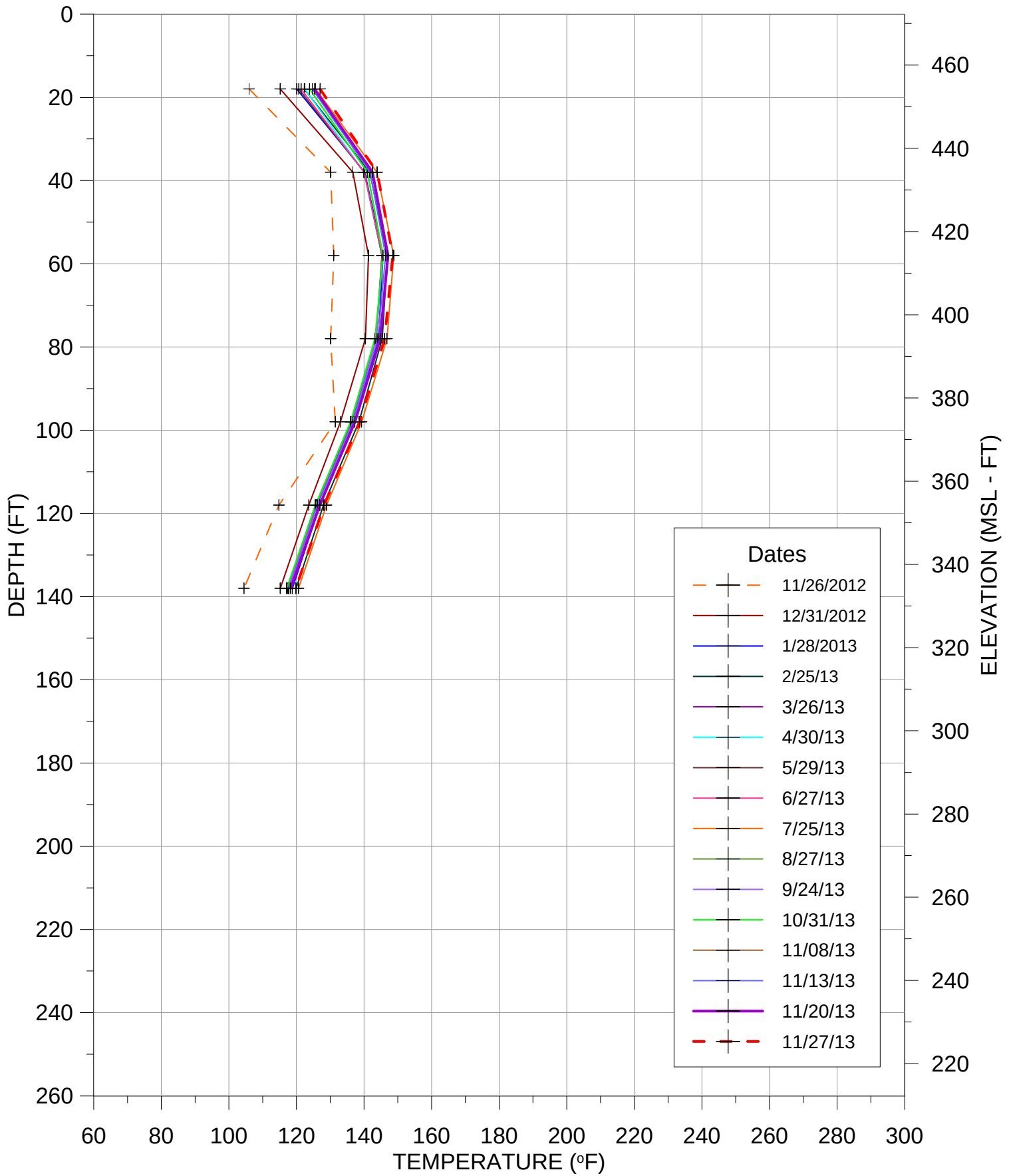
TEMPERATURE VS DEPTH BRIDGETON LANDFILL
