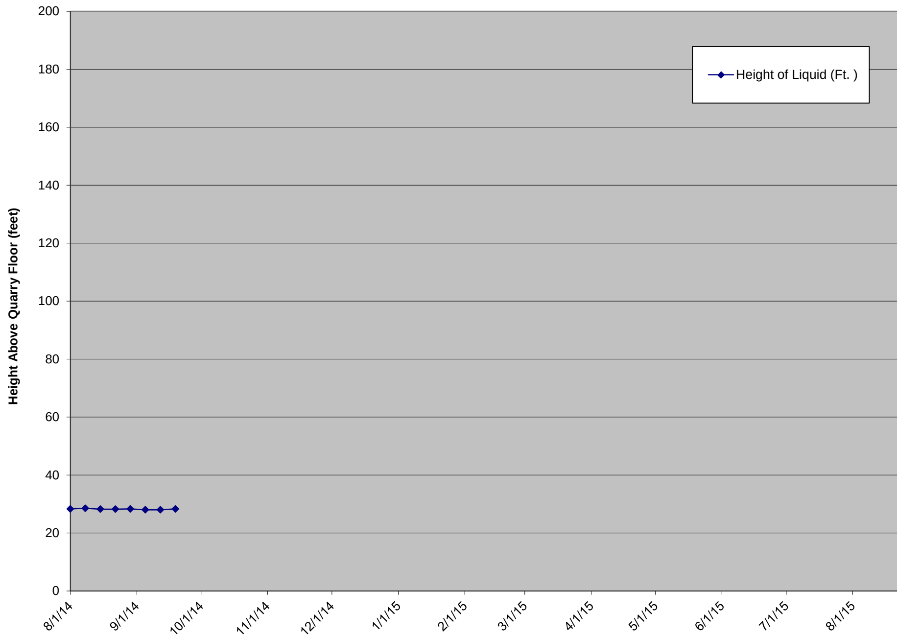
LCS-2D Liquid Level Above Quarry Floor
