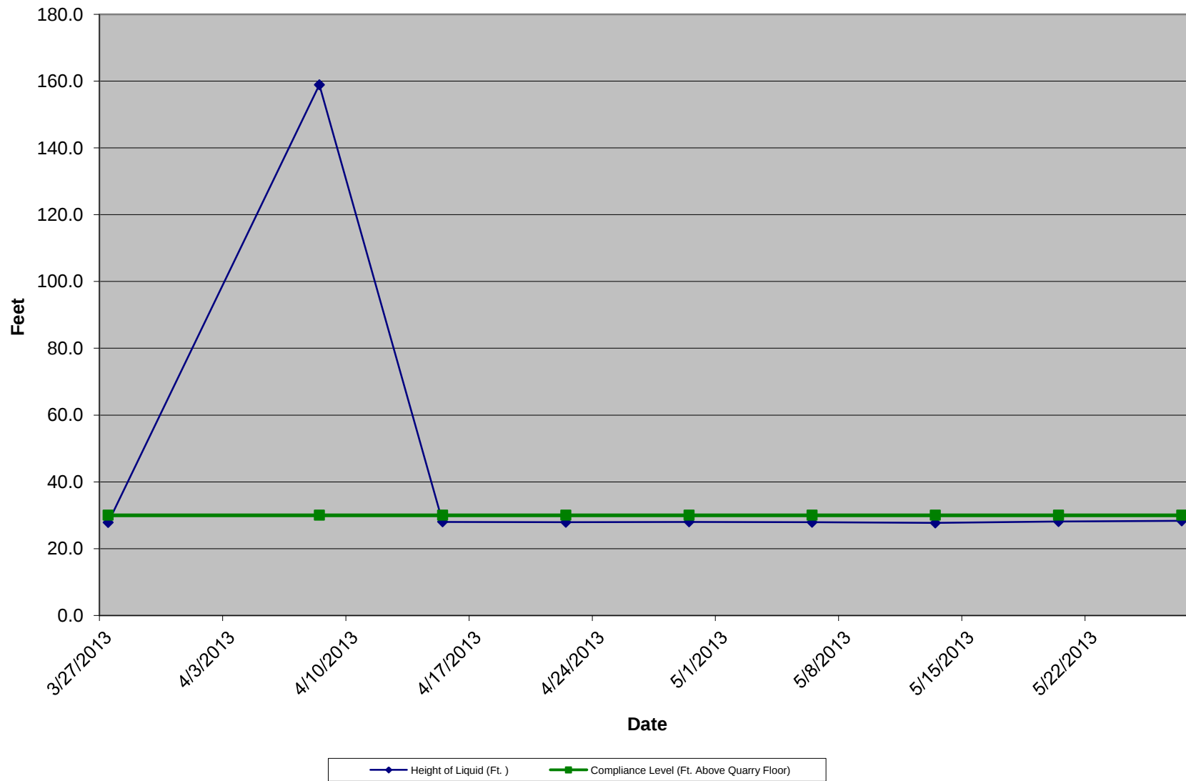
LCS-2D Liquid Level Above Quarry Floor
