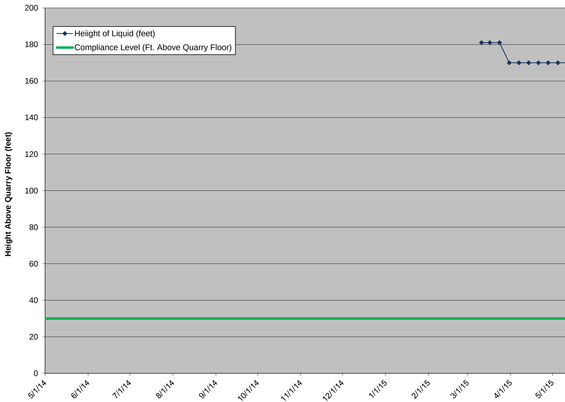
LCS-4B Liquid Level Above Quarry Floor
