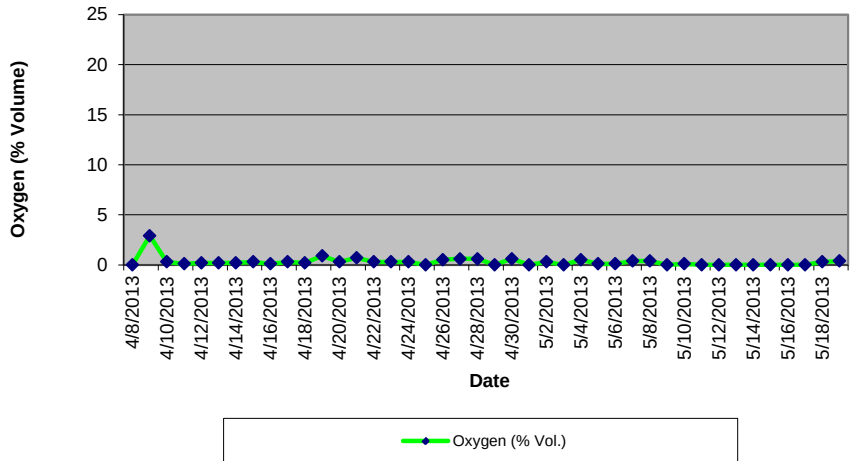
GIW-7 Oxygen (% Volume)
